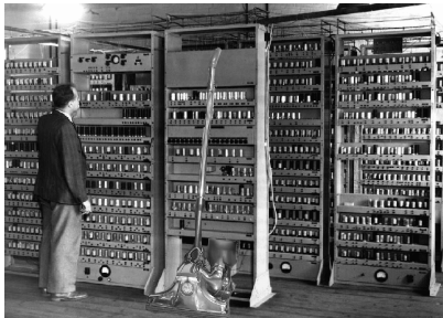
EDVAC-Electronic Discrete Variable Automatic Computer (1949)
